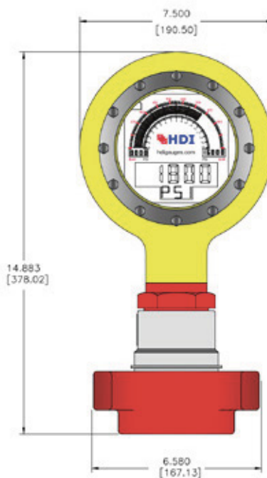
2" 1502 HAMMER UNION SHOWN
