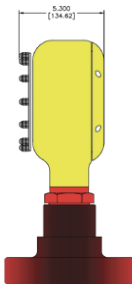
WITH API FLANGE
