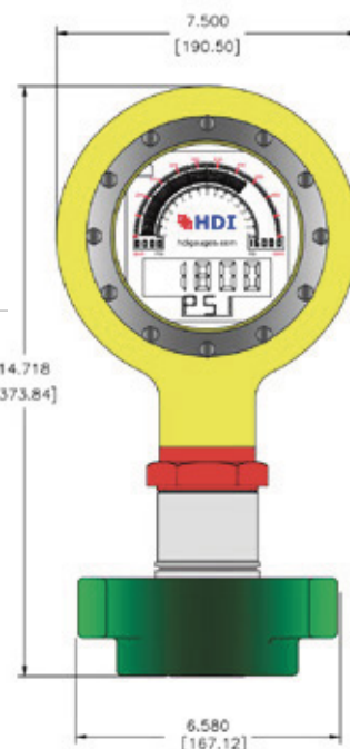
2" 2202 HAMMER UNION SHOWN
