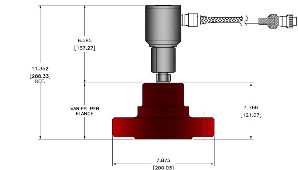
*2-1/16" 10M API FLANGE H2S PSL LEVEL 3 WITH BX152 RING GROOVE SHOWN
