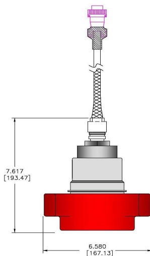
2" 1502 HAMMER UNION SHOWN
